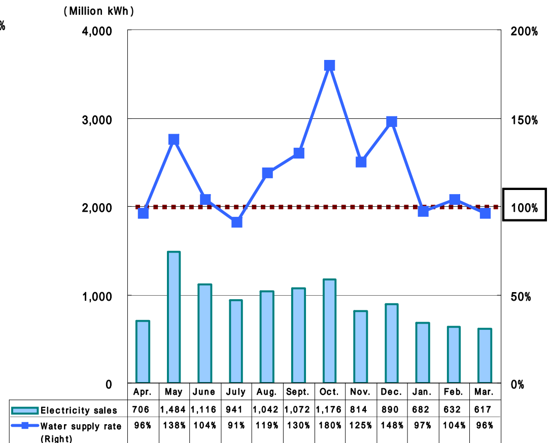
Hydroelectric Power: Monthly Electricity Sales
